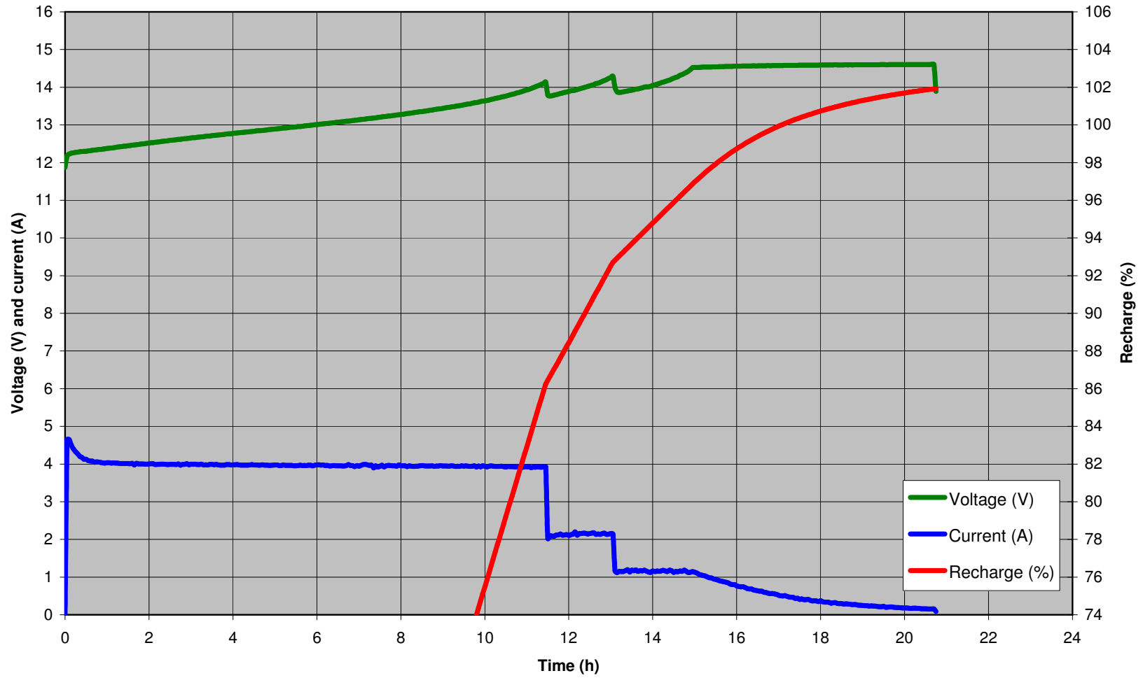
Charger Exide 12/4, 4A Battery: Car (standard wet) 62Ah, discharged 85% Temperature: 20 °C
